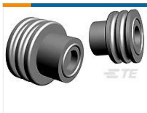
TE 产品编号1823111-1 SINGLE WIRE SEAL, FOR WIRE 2.5 SQMM, BN
