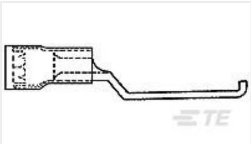
TE 产品编号151793 22-16 LIPPED BLADE EXP.1
