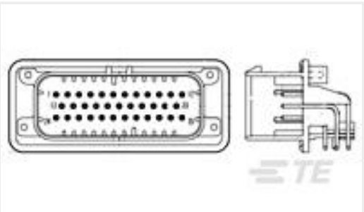
TE 产品编号1-776163-5 35POS,AMPSEAL,PIN HSG ASSY,SLD, COD 5
