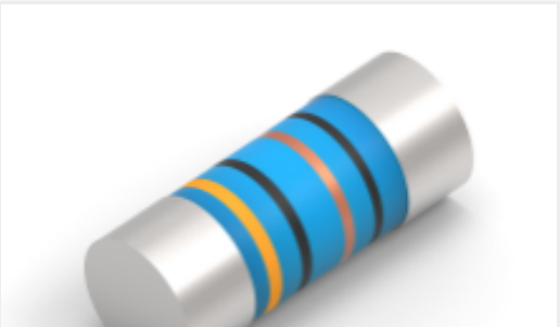
TE 产品编号7-2176314-0 MELF SMA-A 12R 1% 50PPM 0102 0.3 W
