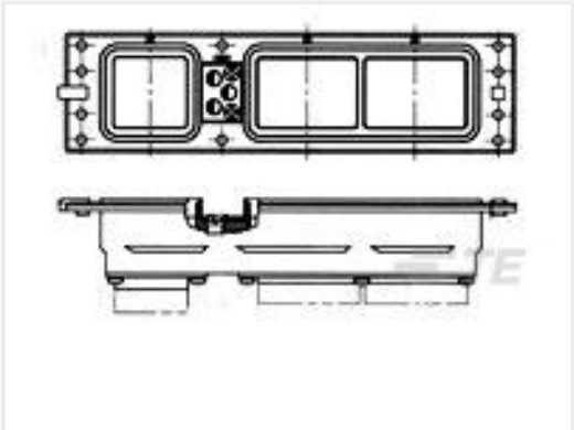
TE 产品编号1-211991-0 RECEPT ASSY, SZ 2, ARINC 600
