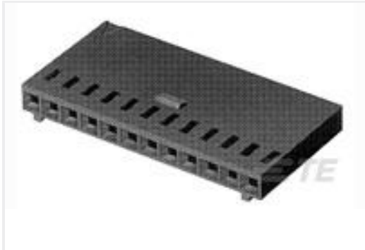
TE 产品编号280359 AMPMODU II REC. HSG, SINGLE ROW, 4 POS.
