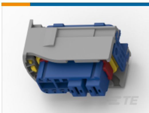
TE 产品编号1-2141564-0 10POS, MIXED,REC HSG,ASSY, SEALED,BU
