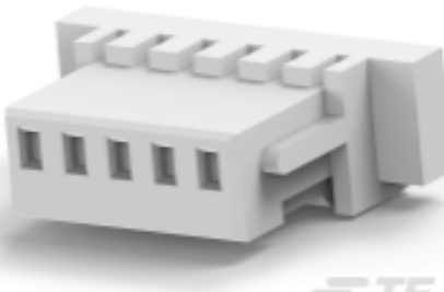
TE 产品编号CAT-H857-H817210 AMP HPI 1.0 mm Receptacle Housings
