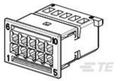
TE 产品编号2-968636-2 10POS MQS REC COD B
