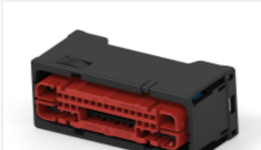
TE 产品编号1-2141968-1 46POS, MIXED, REC HSG, ASSY, SEALED
