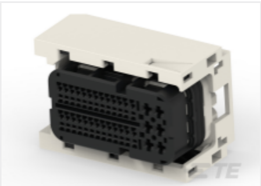
TE 产品编号 9-1563172-9 58POS, MIXED,REC HSG,ASSY
