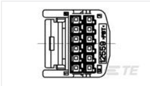
TE 产品编号1746872-1 0.64III 12POS PLUG ASSY
