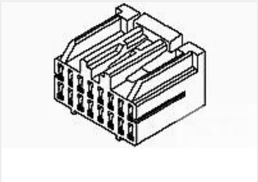
TE 产品编号353212-5 HD HYBRID I/O PLUG ASSY 32P A
