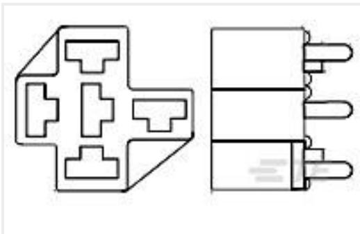
TE 产品编号1393310-3 VCF4-1000=FROM SEC
