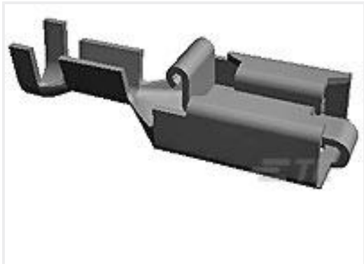
TE 产品编号790319-3 250 PL MKI REC. 12-10AWG PTBR
