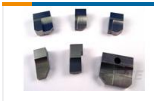
TE 产品编号4-1633932-0 ANVIL, COMBINATION
