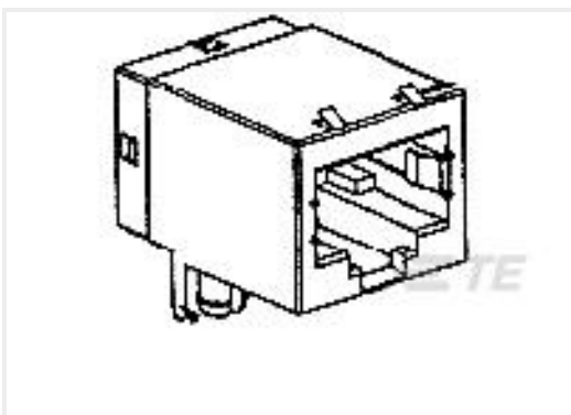
TE 产品编号5558342-1 MJ,8POS,R/A,CAT5,SHLD,PC GND
