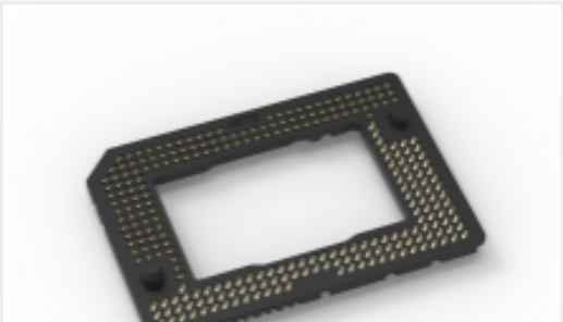
TE 产品编号2319757-1 DUAL LGA,257 POS, DMD SOCKET
