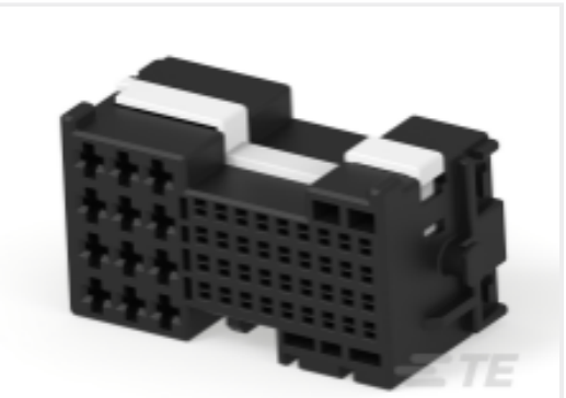
TE 产品编号2109452-2 050/110 48P PLUG ASSY CODE A
