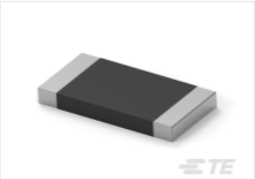
TE 产品编号4-2176421-9 TLRP 2512 2.0W R010 1% 50PPM 4K RL RUG
