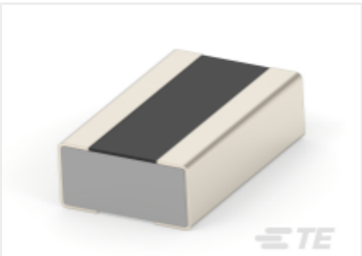
TE 产品编号2176538-1 RLW73P A2 1% R010 600ppm 1k RL
