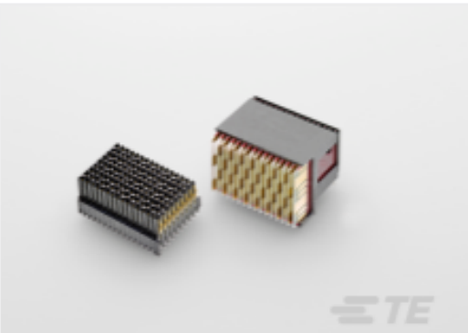
TE 产品编号2302788-2 VERTRECASSY,LEFTEND, HALF, MGRT3
