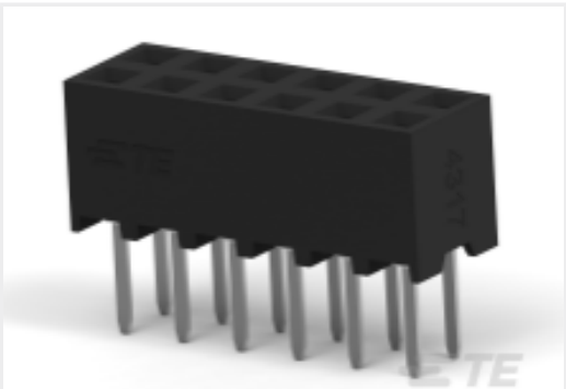
TE 产品编号1-2314822-4 14P,2MM,B-B,REC,DRV,T,2.7,0.76AU,TB
