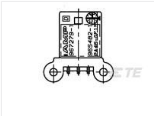
TE 产品编号967279-1 3pos MQS .63 header 90deg THR
