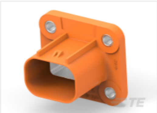
TE 产品编号2310541-2 SPLIT HEADER ASSY, KEY B, HVA280, V0
