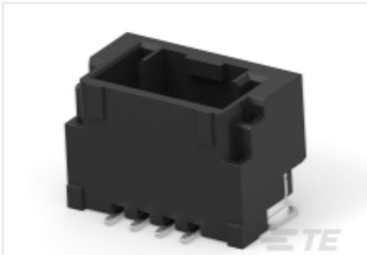
TE 产品编号2-2360540-4 SGI 1.25 HDR, 4P, VT, Key B, Black
