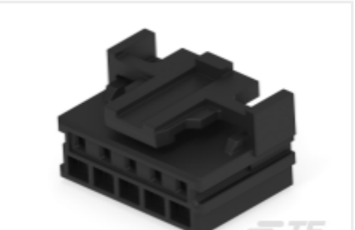
TE 产品编号4-1971030-5 5POS PLUG HOUSING FOR GIC 2.0 EV SERIES
