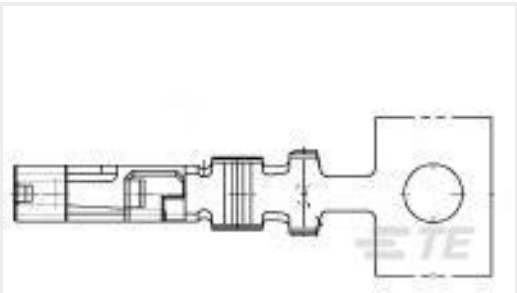
TE 产品编号42563-2 250 FASTON FLAG REC 12-10 AWG TPBR
