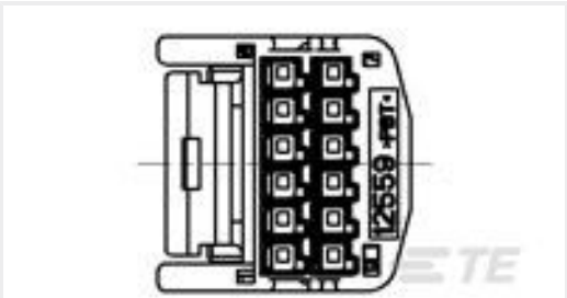
TE 产品编号1746872-1 0.64mm 12POS PLUG ASSY
