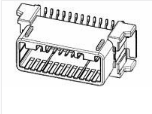
TE 产品编号1717396-2 0.64 SMD 16P CAP ASSEMBLY V-TYPE
