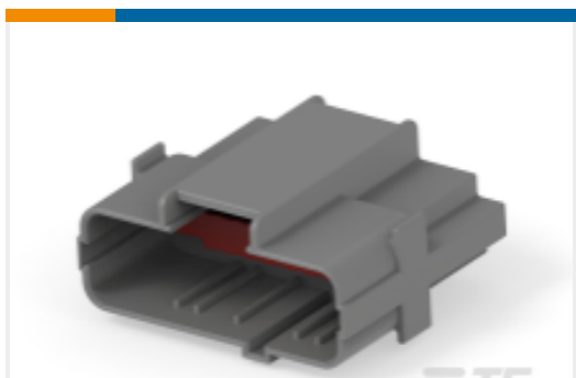
TE 产品编号2098380-2 20 POS HYBRID UNSEALED CAP KY-B STD CLIP
