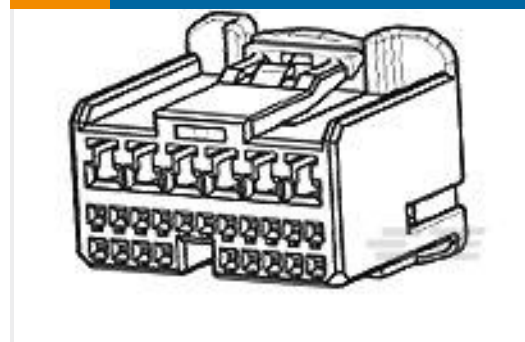
TE 产品编号1318756-1 025/090 ECU PLUG HSG ASSY 24P
