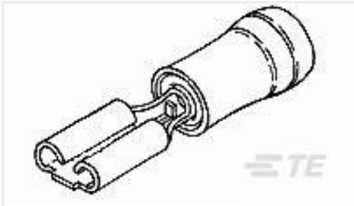
TE 产品编号165616-5 110 PIDG FASTON REC
