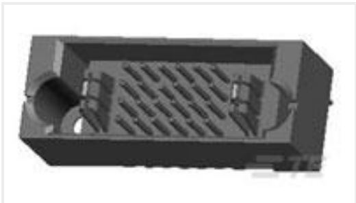
TE 产品编号6450820-2 MBXLE VERT HDR 1P+24S+1P
