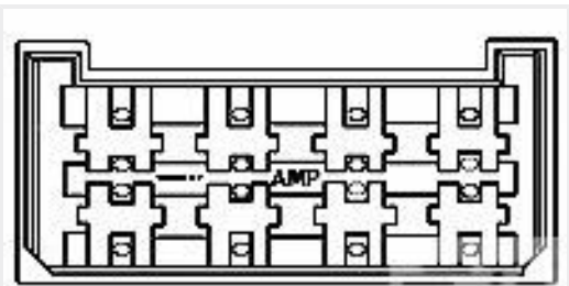
TE 产品编号280099 FF 250 TAB HSG 8P NYLON CLEAR
