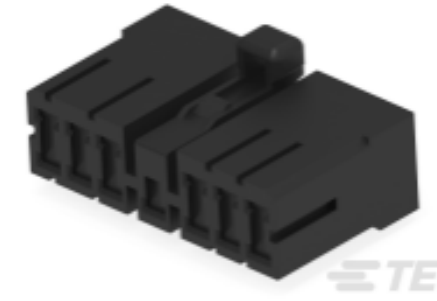
TE 产品编号172498-1 MIC PLUG HSG 13P (MK II)
