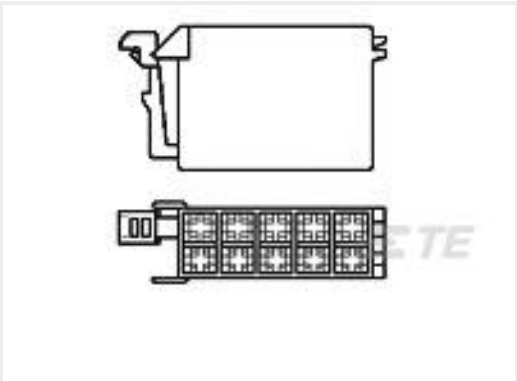
TE 产品编号962190-1 10P JUNIOR-TIMER GH
