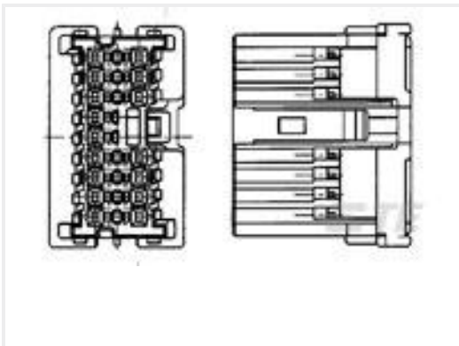
TE 产品编号1123377-6 040 MLC PLUG HSG ASSY 16P
