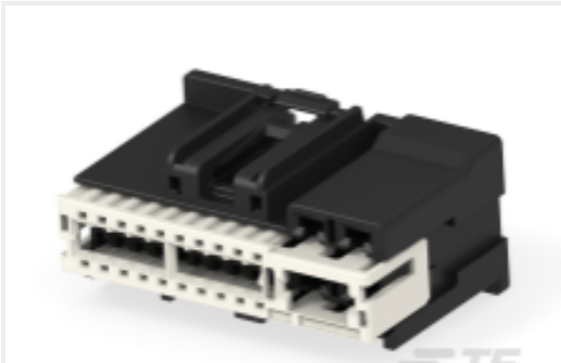
TE 产品编号2288274-1 24P HYBRID 0.64/2.8 PLUG ASSY, A KEY
