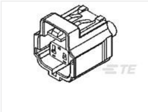
TE 产品编号6-178449-6 EJ-2 DBL LOCK PLUG 2P ASSY
