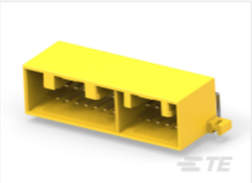
TE 产品编号1-5172491-7 PULSE LOCK CAP HSG ASSY 30P
