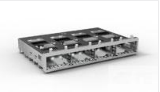
TE 产品编号2007668-1 1x4 QSFP Cage Assy Behind Bzl, LP Holder
