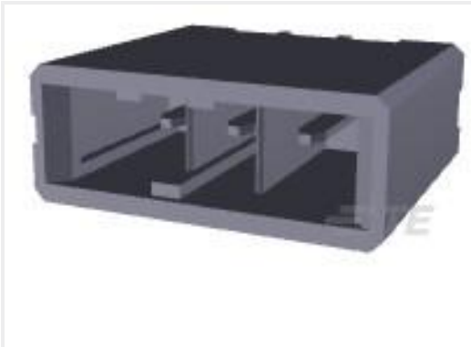
TE 产品编号1-178136-2 DYNAMIC D3200 HDR V ASSY 3P
