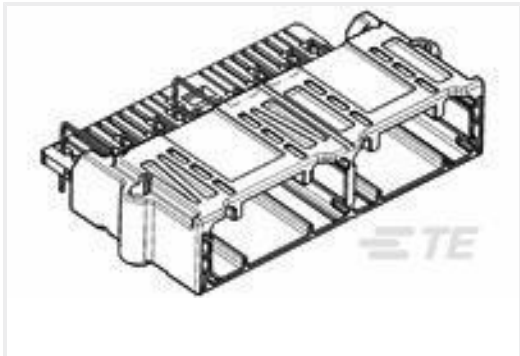
TE 产品编号1939331-1 0.5 30POS CAP ASSY DIP SCREW
