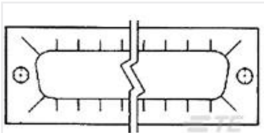
TE 产品编号745776-4 RFI GASKET,SZ 3,PLTD TIN
