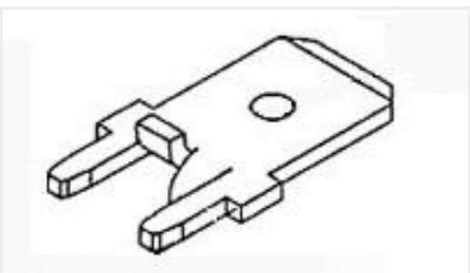
TE 产品编号1217167-1 250 FASTON, PCB TAB, TC BR
