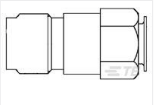
TE 产品编号228636-1 JACK,SMA,SST,.141
