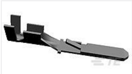
TE 产品编号160743-4 110 FASTIN FASTON,TAB,20-16 AWG, PTBR
