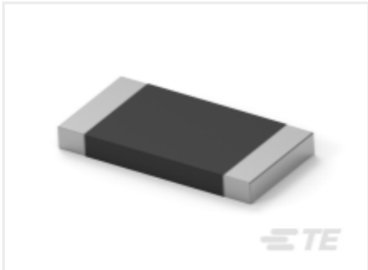
TE 产品编号8-2176422-2 TLRP 2512 3.0W R005 1% 75PPM 4K RL
