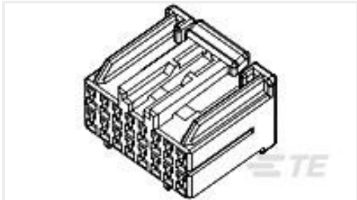
TE 产品编号917989-1 HYBRID MK-2 PLUG HSG ASSY 22P
