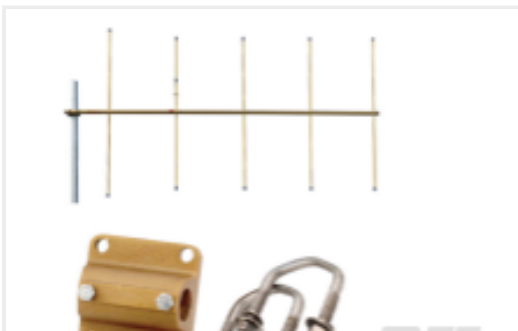
TE 产品编号Y1505 YAGI, GLD, 5, 150-174 MHz 9.2dBi
