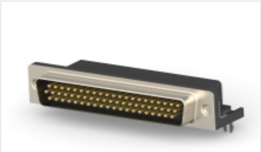
TE 产品编号2311773-1 AMPL PLUG, HD22, R/A, 62P, THREADED
