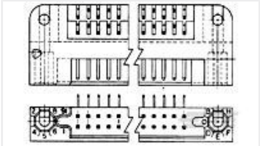
TE 产品编号531720-8 2 ROW BOX PIN 80 POS R/A
