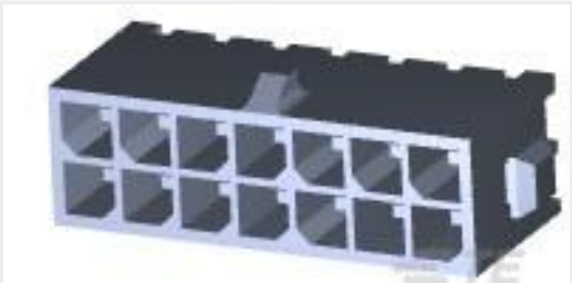
TE 产品编号4-794631-4 14P MICRO MNL ASSY,VRT,HDR LF
